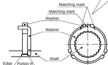
C Detail of installation of washer
