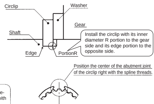
B Detail of installation of circlip
