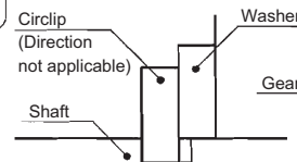
B Detail of installation of circlip
